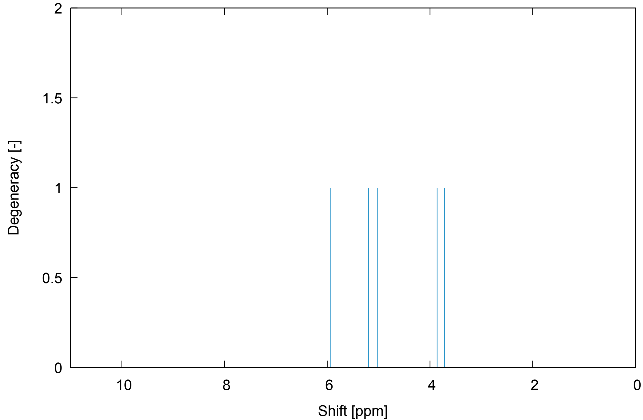
NMR spectrum for H of compound at b3lyp/6-311+G(2d,p)
